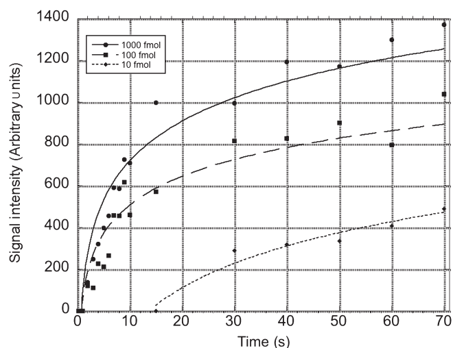
Figure 6. Time course of LFM detection: 10- \mu l samples containing either 1000 fmol (circle), 100 fmol (square) or 10 fmol (diamond) dnaR89 were run on appropriately patterned LFMs. Video data were collected and colorimetric signal intensity measured from video frames at R-77-96 capture features. Capillary transport of the 10- \mu l sample was complete by 120 s. Lines represent logarithmic curve fits to the data.
